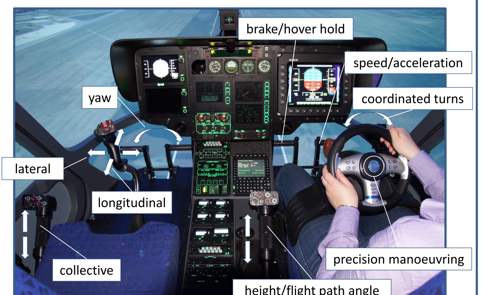
AVES helicopter cockpit with conventional inceptors on the left side and steering wheel control on the right.
